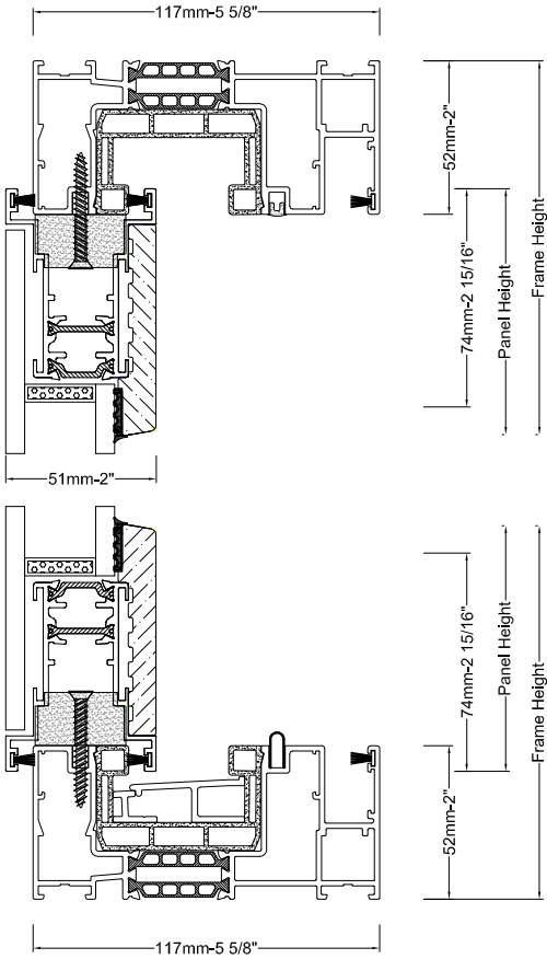
Section 1: Fixed Panel
